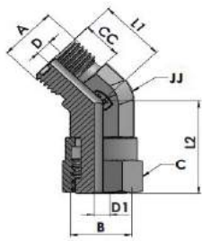
XXHTFS6502-00-00 Series MFS-FFSS 45° ELBOW
