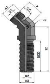
XXHTFS2702-00-00 Series MFS-MFS BULKHEAD 45° ELBOW
