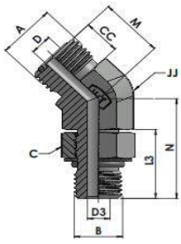
XXHTFS7300-00-00 Series MFS-MMAORB 45° ELBOW
