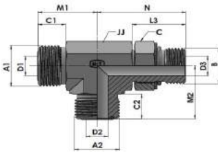
XXHTFS7215-00-00 Series MFS-MMAORB-MFS TEE
