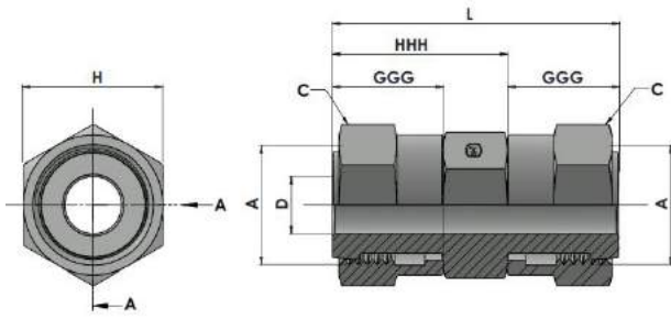
XXHTFS6565-00-00 Series MFS-MORB STRAIGHT LONG
